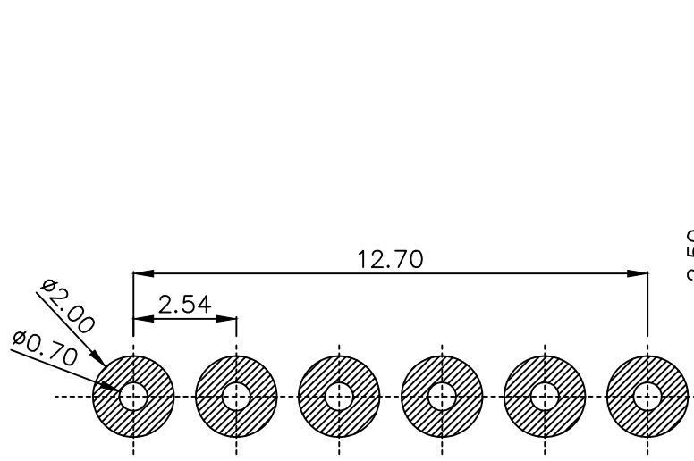
Recommended pcb layout Layout tolerance: ±0.05mm
